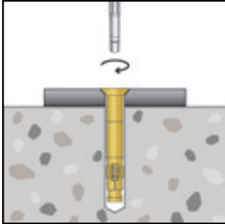
Install the refreshed anchor according to its' installation instruction.
