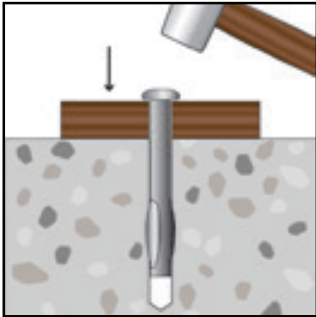
Place fixture then drive anchor through fixture into drilled hole using a hammer until fixture is firmly clamped.
