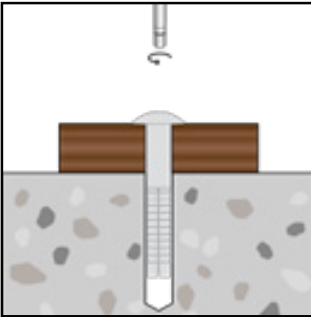
Anchor may be removed by unscrewing drive pin with a flat blade screwdriver.
