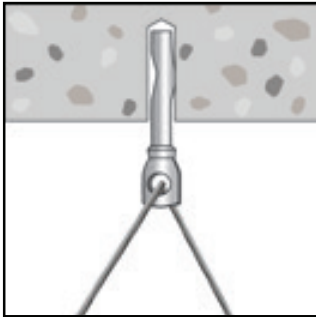
Affix cable/wire through the anchor eyelet and secure.
