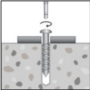
Insert anchor through fixture into the drilled hole. Drive using the nominated driver bit whilst applying constant forward pressure until fixture is clamped.
