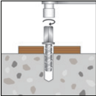
Insert anchor into hole and screw in using spanner, socket or an impact wrench. Apply constant forward pressure when driving and tighten until the fixture is firmly clamped.
