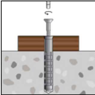
Screw may be removed later if required, using a screwdriver.
