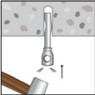
Drive anchor into drilled hole to the required embedment depth.
